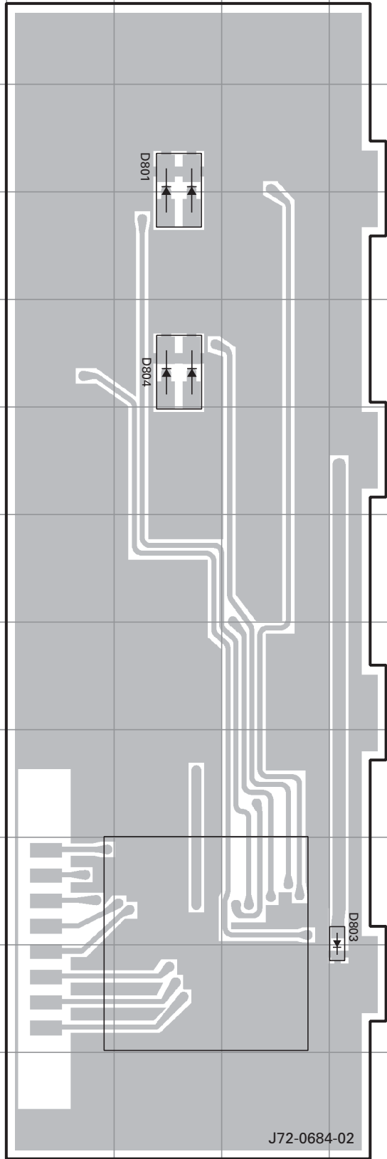
DISPLAY UNIT (X54-3280-10) Component side view (J72-0684-02)
