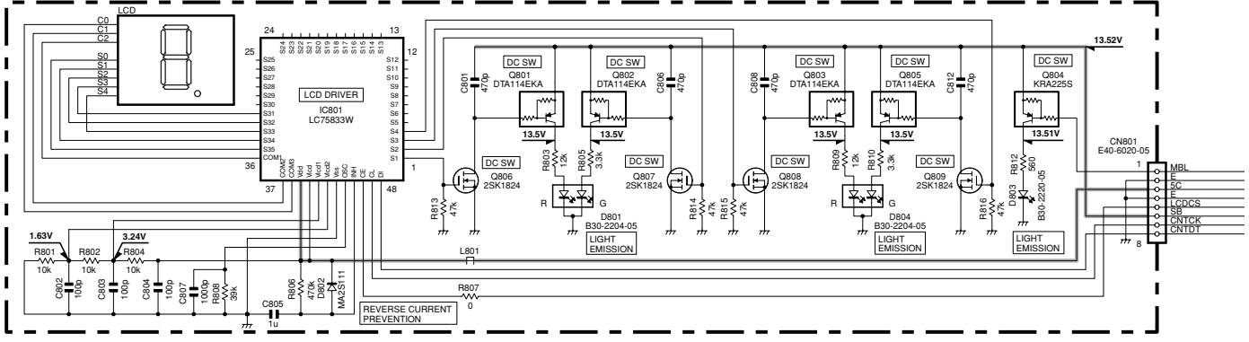
CONTROL UNIT (X57-5963-02) (B/2)
