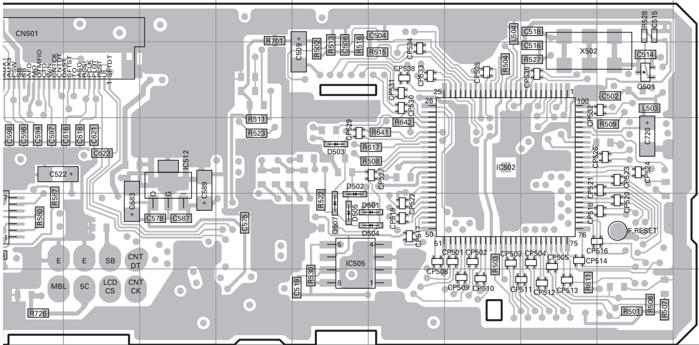
TX-RX UNIT (X57-5963-02) (B/2) Foil side view (J72-0988-09 B/2)
