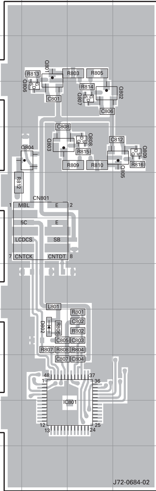
DISPLAY UNIT (X54-3280-10) Foil side view (J72-0684-02)
