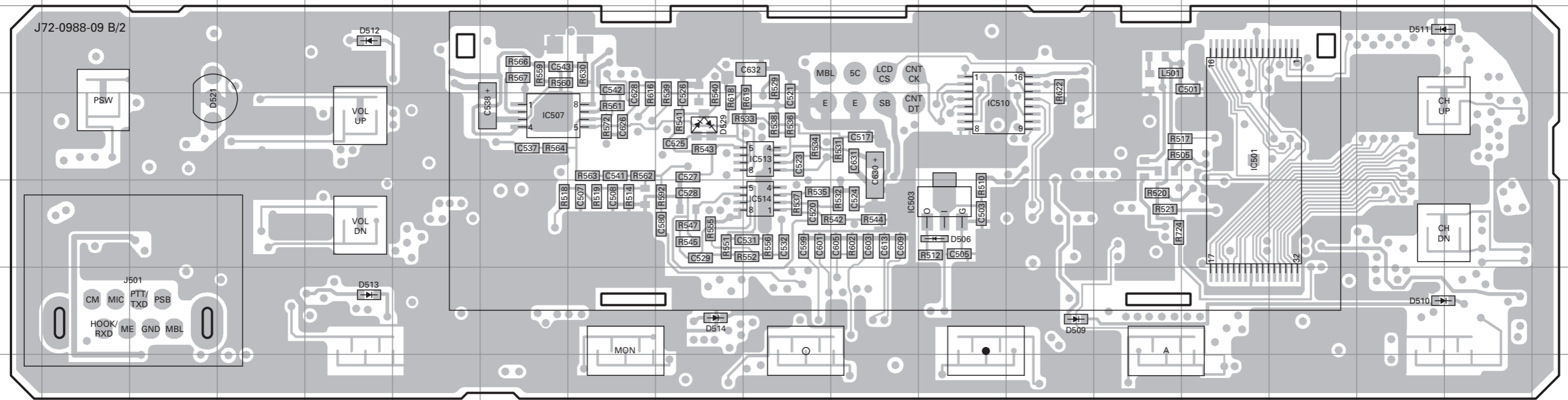
TX-RX UNIT (X57-5963-02) (B/2) Component side view (J72-0988-09 B/2)
