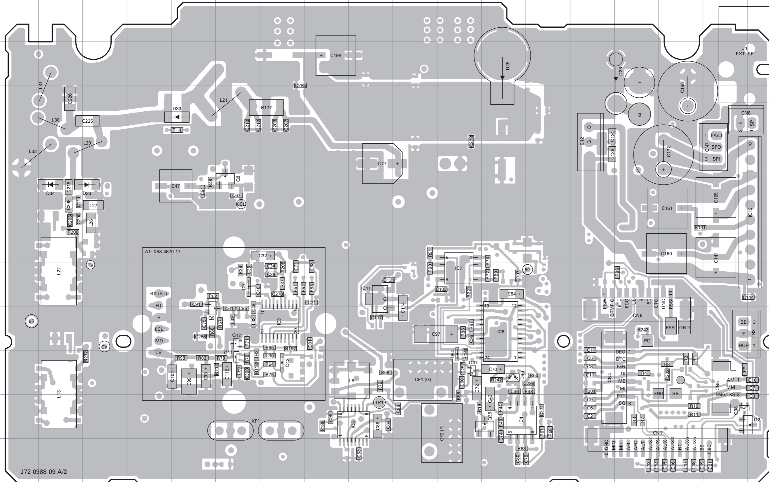
TX-RX UNIT (X57-5963-02) (A/2) Component side view (J72-0988-09 A/2)
