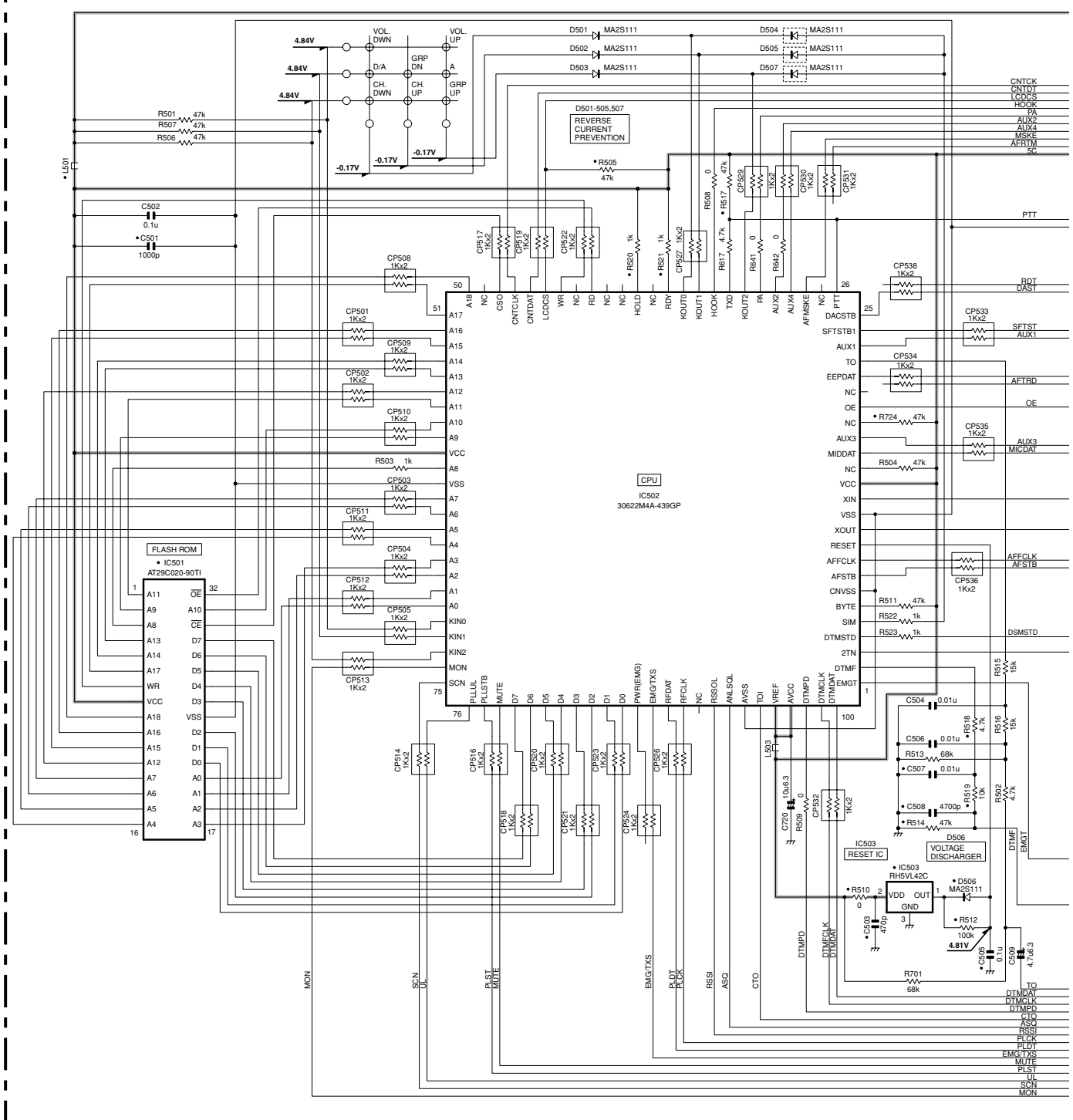
CONTROL UNIT (X57-5963-02) (B/2)
