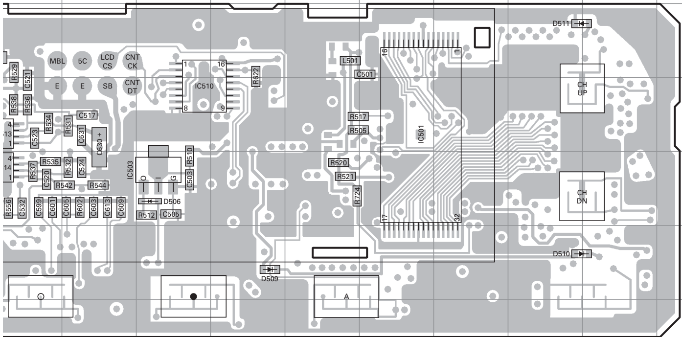
TX-RX UNIT (X57-5963-02) (B/2) Component side view (J72-0988-09 B/2)
