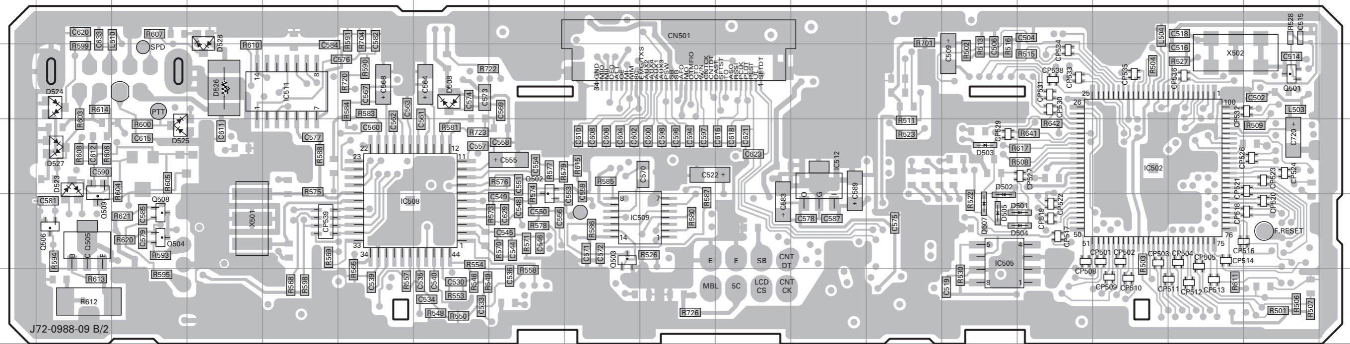
TX-RX UNIT (X57-5963-02) (B/2) Foil side view (J72-0988-09 B/2)
